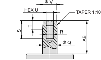
Piston rod end detail for double-sided arm:
