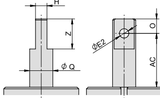
Piston rod end detail for double-sided arm:
